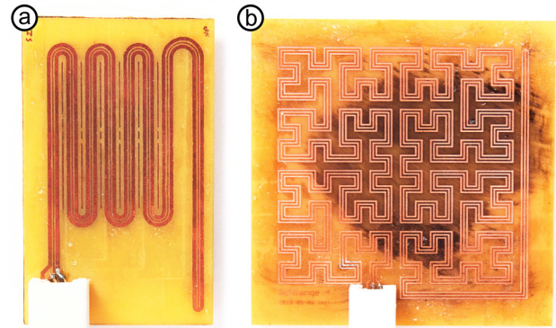
Figure 12: We touch-enabled surfaces not (a) using serpentines but (b) using Hilbert curves. In both prototypes, traces are spaced 5mm apart, so that a finger touches at least two different locations along the trace.
