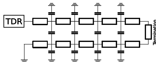
Figure 2: Lumped circuit model of wire pair connected to a time domain reflectometer. Each wire is capacitively coupled to the environment and to the other wire.
