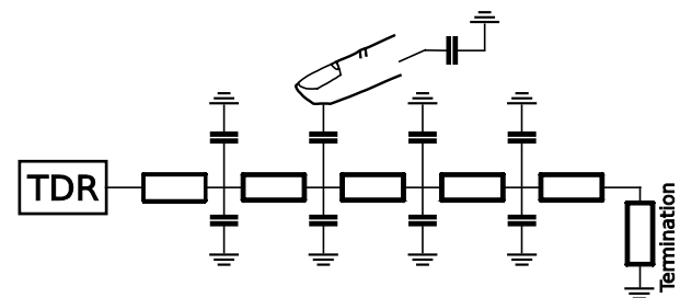
Figure 7: A lumped circuit model of a single wire touch-enabled using TDR. Touching the wire increases its capacitive coupling to the environment at the touch location.
