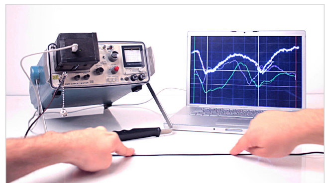
Figure 5: Our experimental setup is based on a Tektronix 1502 reflectometer built in 1975.
