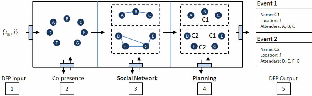
Figure 3. Data fusion method 1; illustrating how the method uses the enablers to group co-present users into subgraphs using social ties, before analysing planning data within each subgroup to create events. DFP = Data Fusion Process
